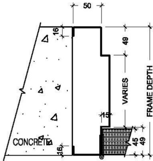
DOUBLE RABBETS WELDED TYPE FRAME
